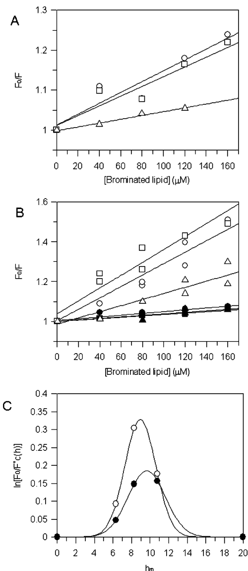
FIGURE 4: Stern–Volmer plots for the depth-dependent quenching of Trp fluorescence for (A) WT ECP and (B) W10K (○, □, and △) and W35A mutants (●, ■, and ▲). Liposomes containing 3:2 DOPC/DOPG lipids were mixed with an increasing molar ratio of (6,7)-Br 2 PC (□), (9,10)-Br 2 PC (○), or (11,12)-Br 2 PC (△). Assay conditions were 0.5 \mu M final protein concentration and 200 \mu M liposome concentration. (C) Depth-dependent fluorescence quenching profile of WT ECP (●) and W10K (○) calculated by the DA to visualize the changes in fluorescence Trp chromophores ( F ), normalized to its value in the absence of quenching ( F_0 ), when the quencher is present at certain depths in the bilayer. h_m is the average location depth of the Trp residues.
